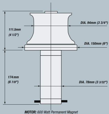
MOTOR: 600 Watt Permanent Magnet
